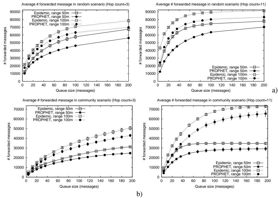
Fig. 7. Communication overhead. a) random mobility scenario b) community scenario
